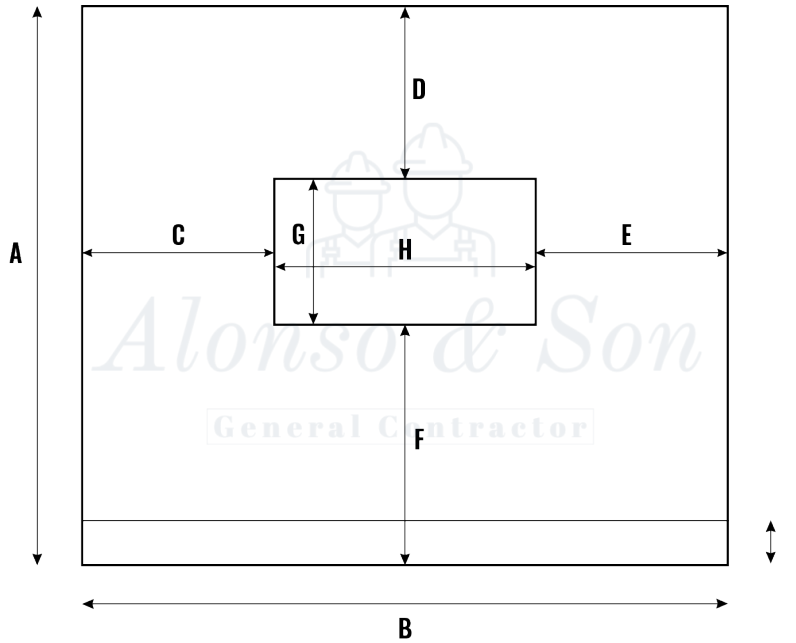
Type: Wall with Window Elevation
